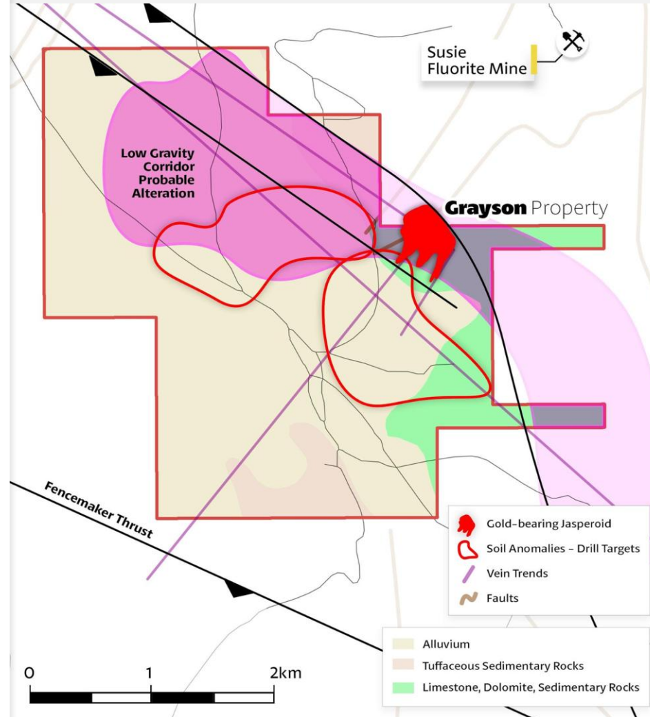
Thrust Faults
